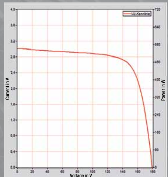
IU characteristic curve
